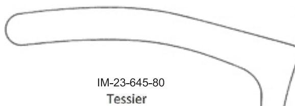
ZI-25-263-60 Tessier 17cm 6 3/4" Nasal Speculum blades 70 x 8,5 mm for adults for dilation, black chromium-plated
