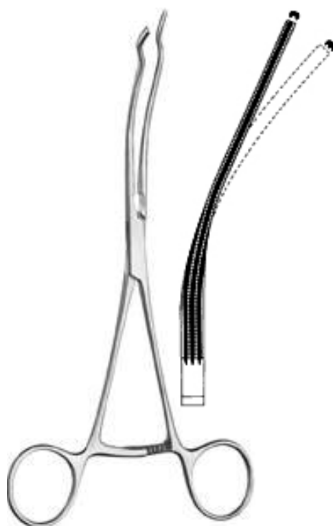
IM-23-570-R Obwegeser 21cm 8 1/4" Fragment Adapting Forceps jaw length 80 mm right
